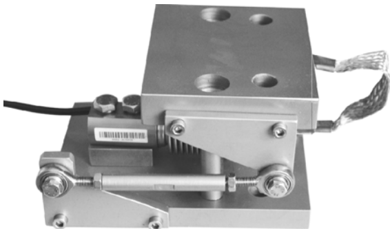
Stainless steel, assembled with: BM11,HM11
